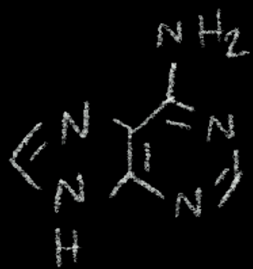
Adenine
