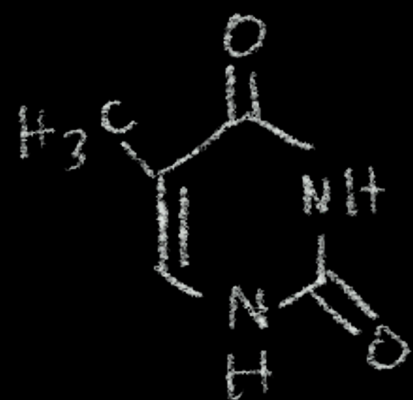
Thymine
