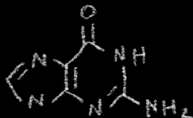
Guanine
